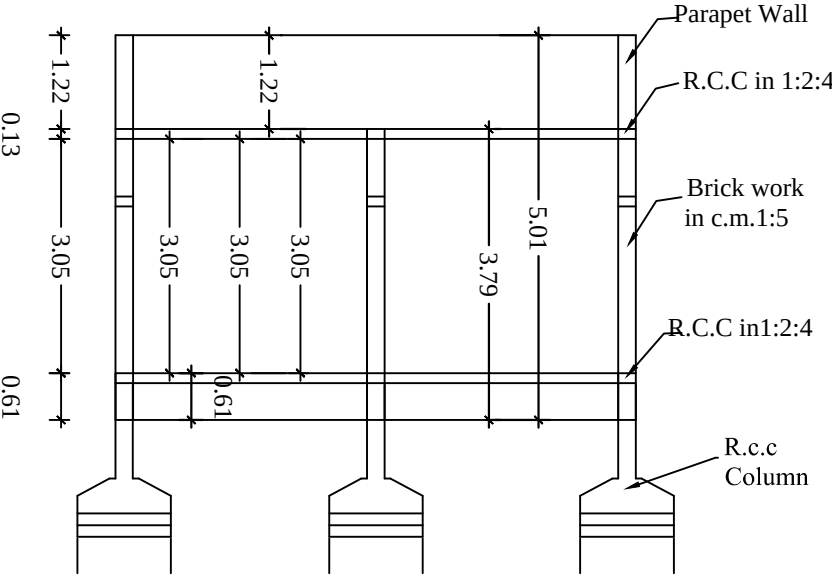
CROSS SECTION-AA
