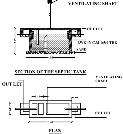
SEPTIC TANK
