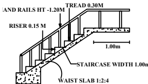
STAIRCASE DETAILS
