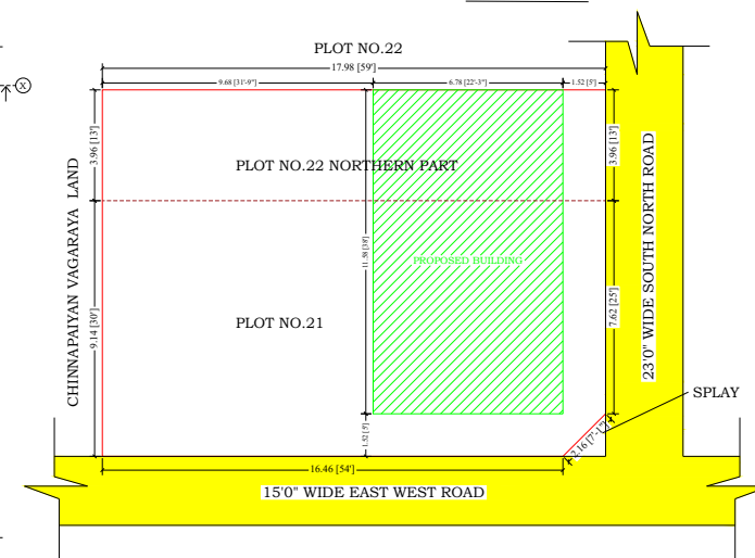
SITE PLAN (SCALE - 1:250)
