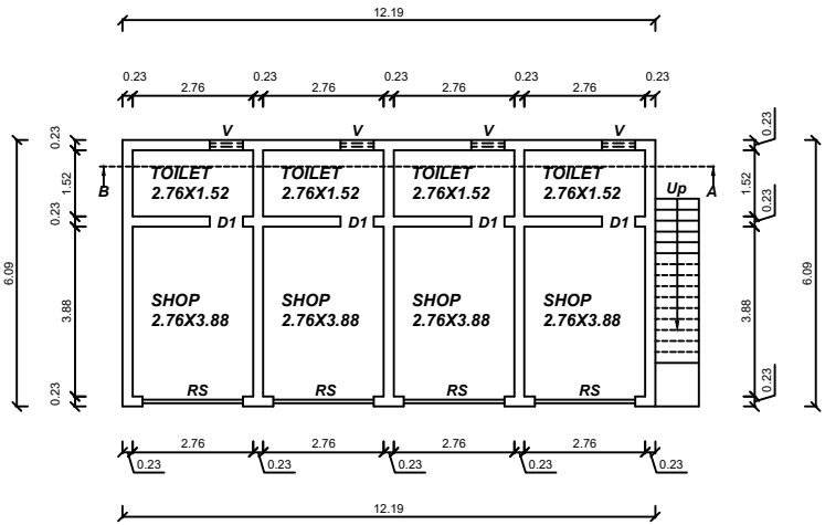
PROPOSED GROUND FLOOR PLAN [Ground Floor Plan]
