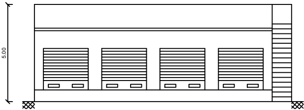
FRONT ELEVATION
