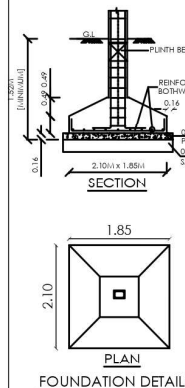
FOUNDATION DETAILS
