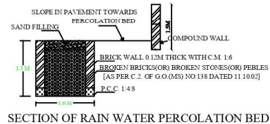
SECTION OF RAIN WATER PERCOLATION BED
