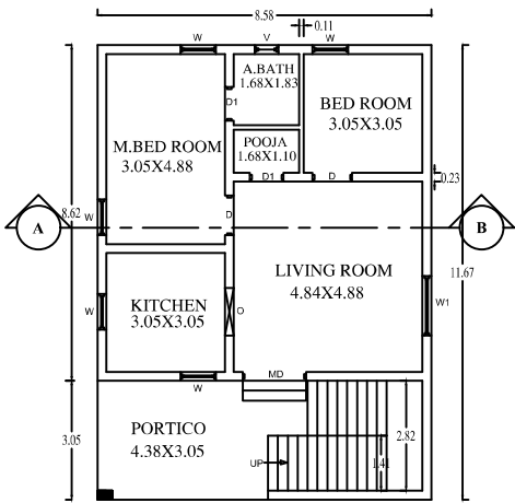
PROPOSED BUILDING OF GROUND FLOOR
