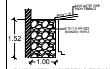
RAINWATER HARVESTING TRENCH
