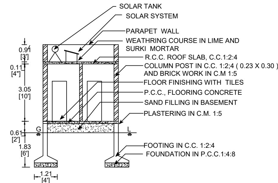
SECTION ON " S P "
