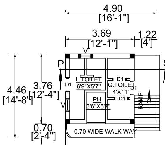
GROUND FLOOR PLAN (TOILET BLOCK)
