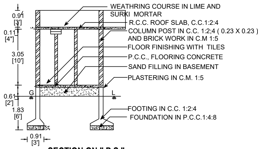
SECTION ON " P S "
