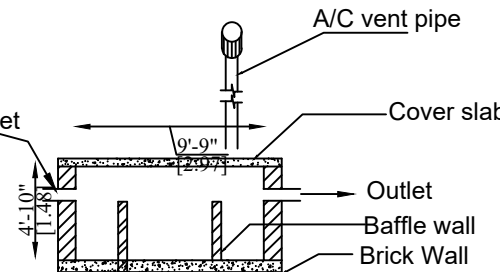
SECTION SS
