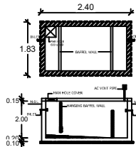
PLAN OF SEPTIC TANK
