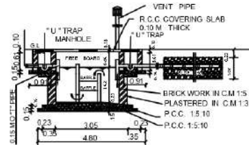
LONGITUDINAL SECTION IN "XX"
