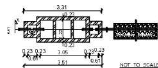
LONGITUDINAL SECTION IN "XX"
