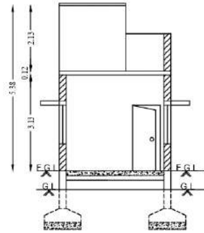
SECTION ON-AA
