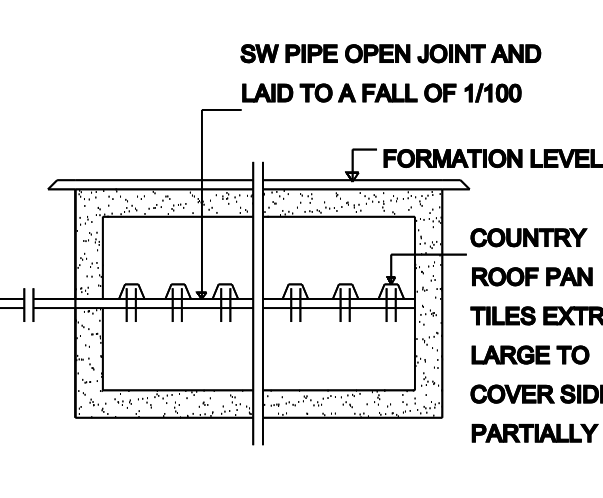
SECTION OF DISPERSION TRENCH
