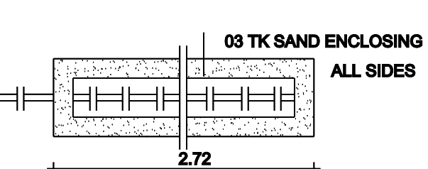
PLAN OF DISPERSION TRENCH
