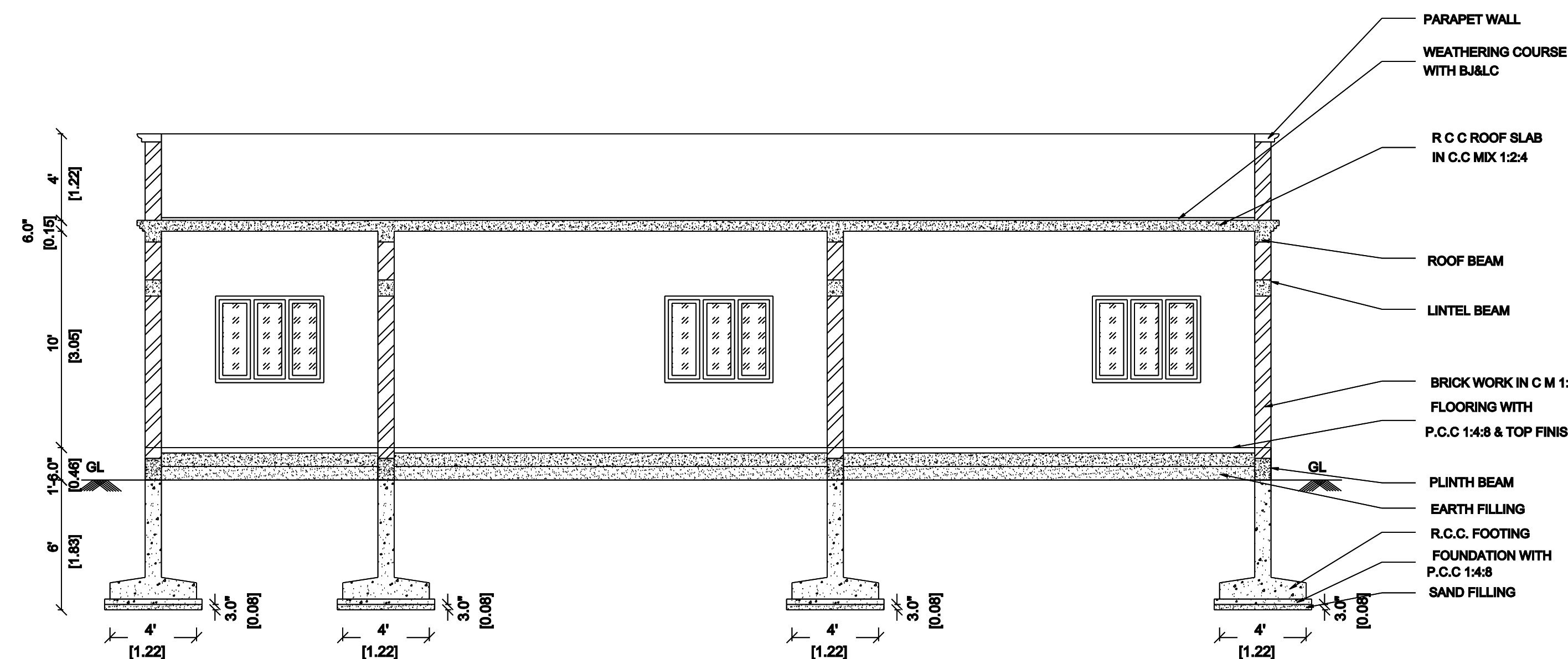
SECTION - 'A-A'
