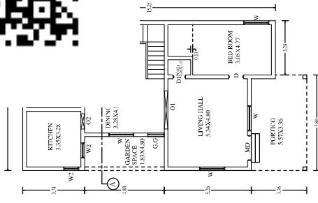
PROPOSED BUILDING OF GROUND FLOOR
