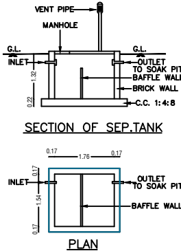
SEPTIC TANK
