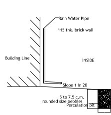
PERCOLATION PIT
