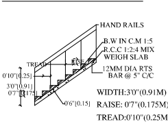
STAIR CASE DETAILS:-
