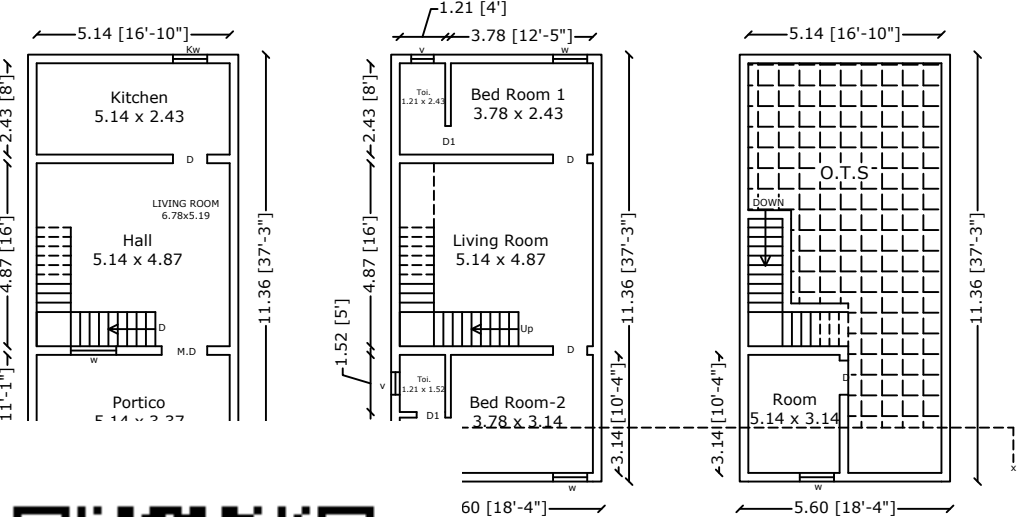
FLOOR PLAN
