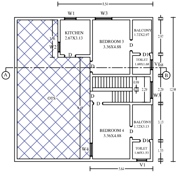
PROPOSED BUILDING OF FIRST FLOOR
