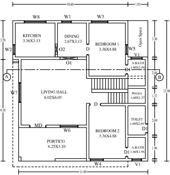
PROPOSED BUILDING OF GROUND FLOOR
