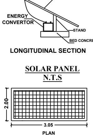
SOLAR BOARD
