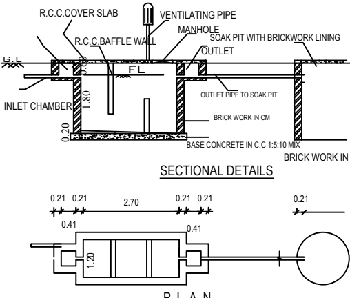
DETAILS OF SEPTIC TANK WITH SOAKPIT
