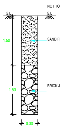
RAIN WATER PERCUSSION PIT
