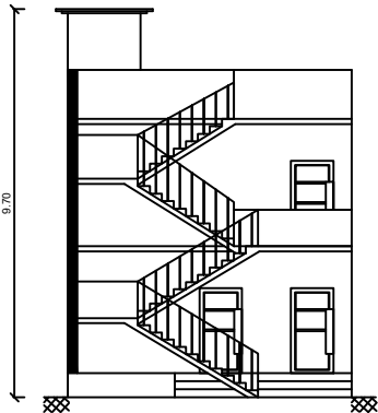
FRONT ELEVATION
