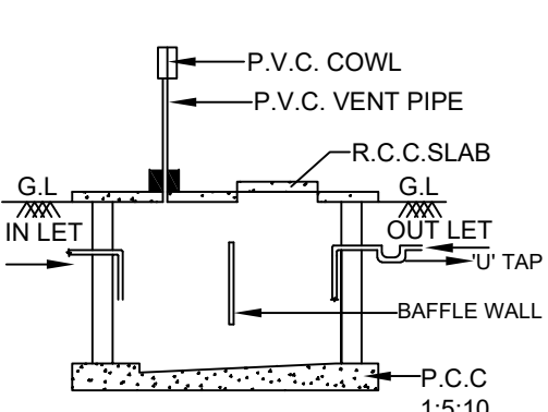
SEC. OF SEPTIC TANK
