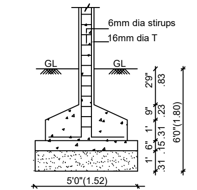
COLUMN FOUNDATION DETAIL
