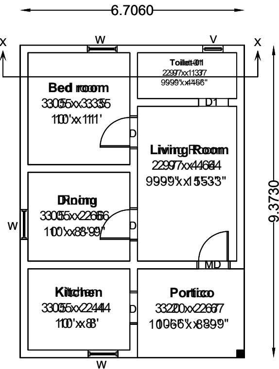
SITE CUM PRO.GROUND FLOOR
