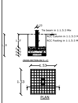
COLUMN FOUNDATION DETAILS:-
