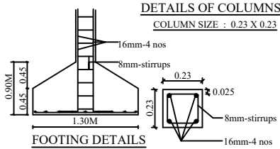
SCALE - 1 : 100 ALL DIMENSIONS ARE IN METER
