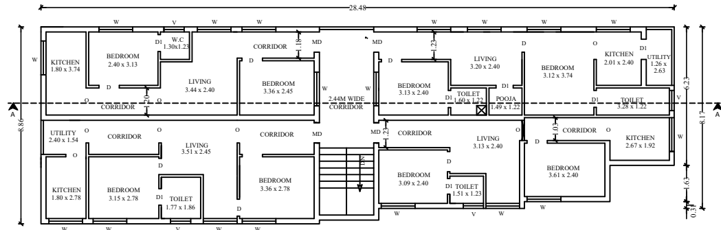
PROPOSED FIRST FLOOR PLAN (SCALE 1:100)
