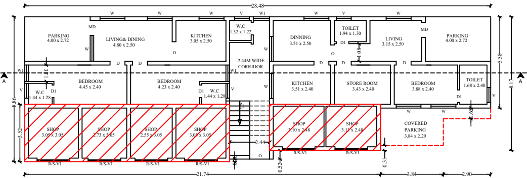
PROPOSED GROUND FLOOR PLAN WITH APPROVED COMMERCIAL SPACE IN GROUND FLOOR [APPROVED NO FOR COMMERCIAL SPACE - ROC NO : 596/2025, BA NO : 4/2025-2026] (SCALE 1:100)
