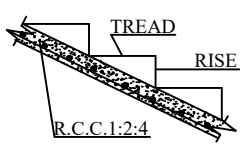
STAIR DETAILS
