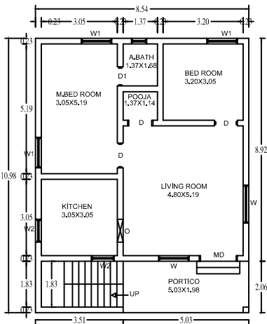
PROPOSED BUILDING OF GROUND FLOOR
