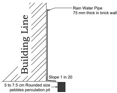
RAINWATER HARVESTING
