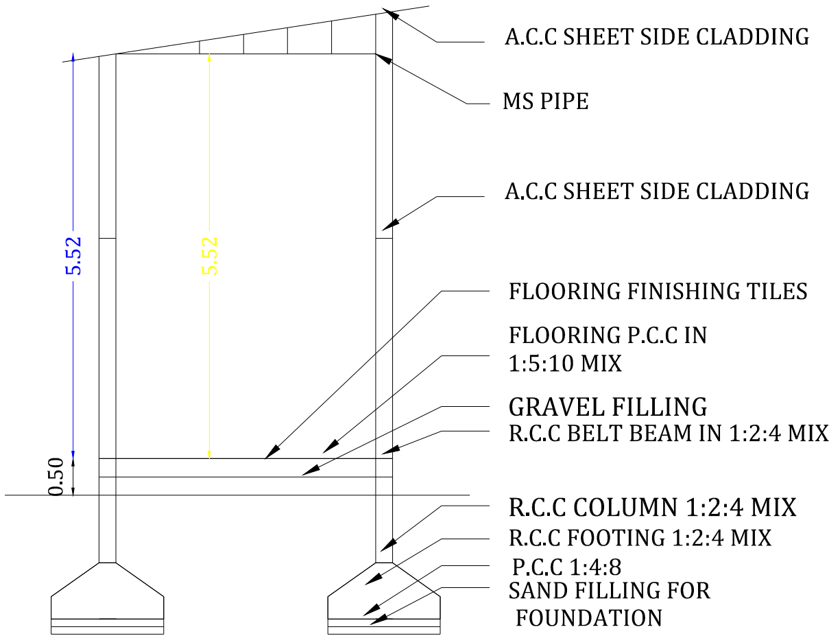
SECTION A TO B
