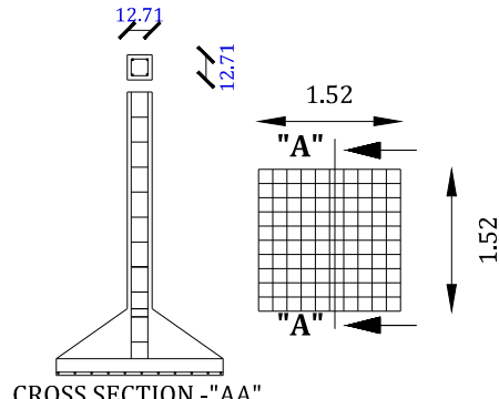
COLUMN DETAILS :-
