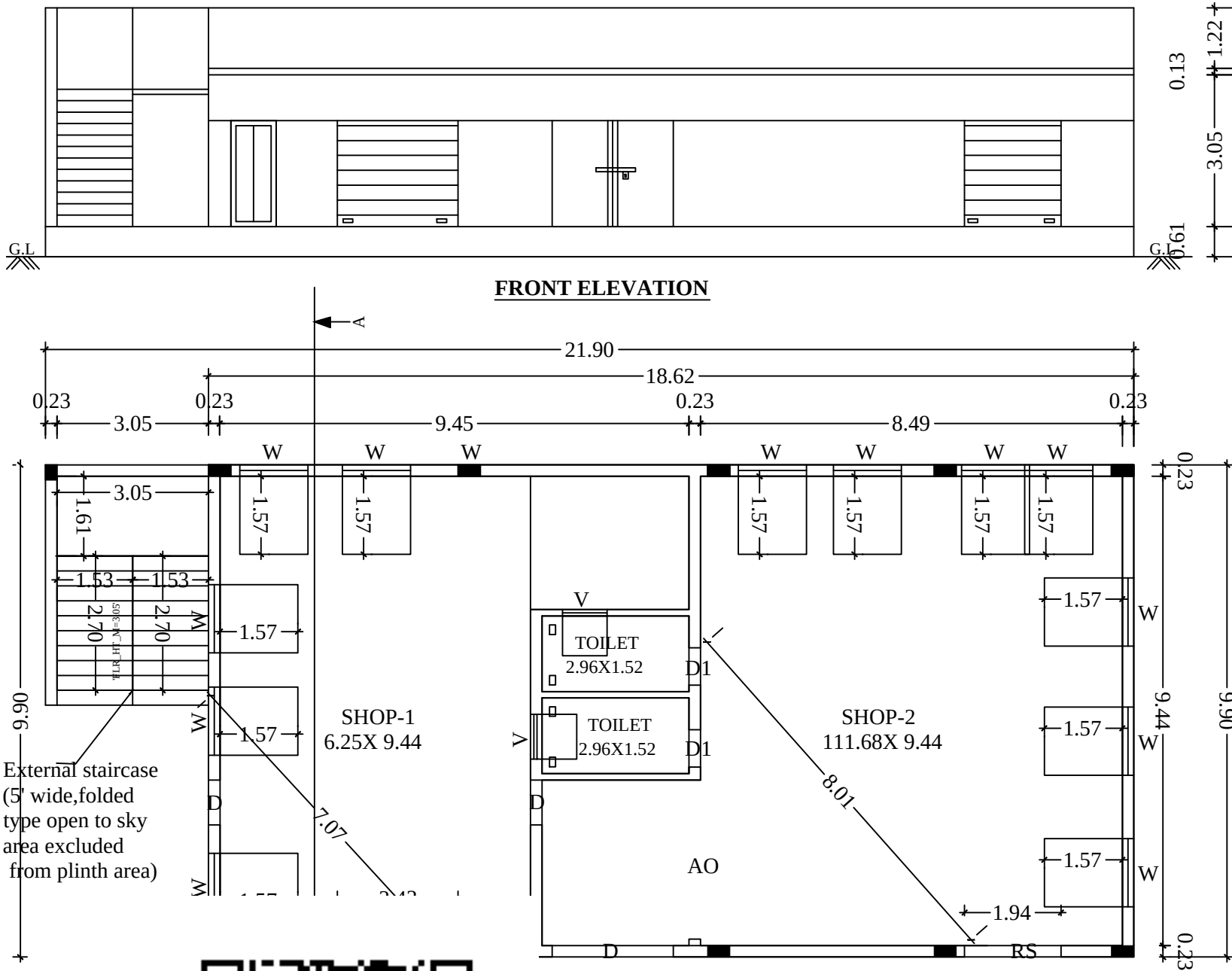
PLAN FOR GROUND FLOOR
