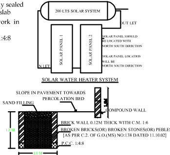
SECTION OF RAIN WATER PERCOLATION BED
