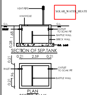
SEPTIC TANK
