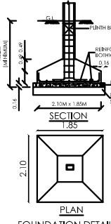
FOUNDATION DETAILS
