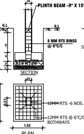
COLUMN & FOOTING DETAIL
