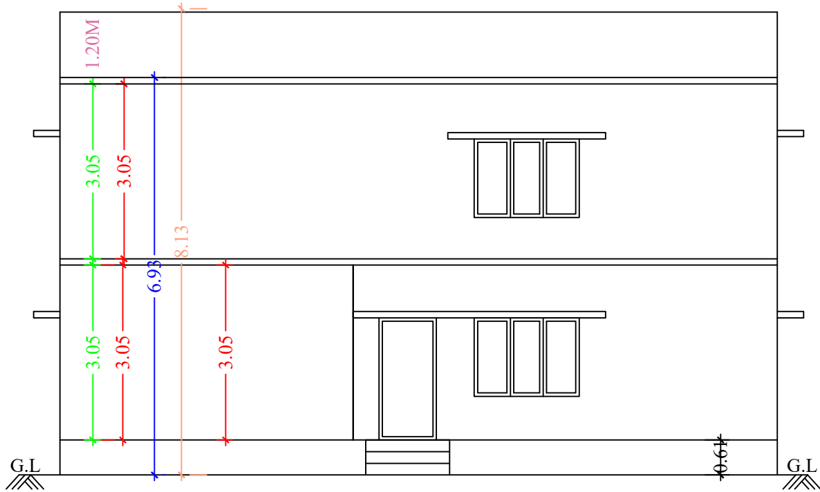
FRONT ELEVATION
