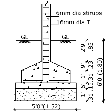
COLUMN FOUNDATION DETAIL
