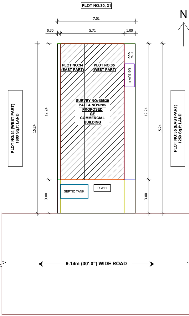
SITE PLAN
