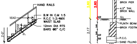
STAIRCASE DETAILS
