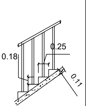
STAIRCASE DETAILS:-
