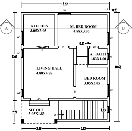
PROPOSED BUILDING OF GROUND FLOOR
