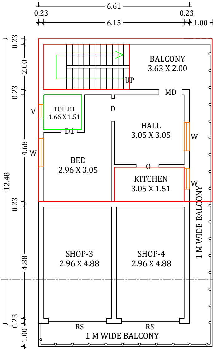
EXISITNG AND PROPOSED FIRST FLOOR PLAN
