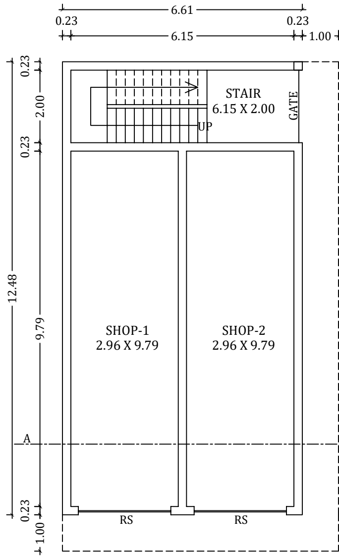
EXISITNG GROUND FLOOR PLAN
