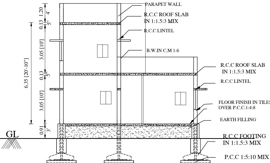
SECTION ON -AAA
