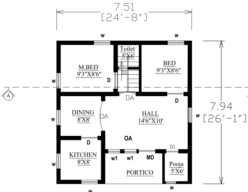
GROUND FLOOR PLAN FACED TO EAST
