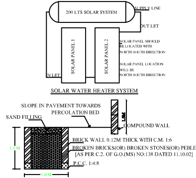
SECTION OF RAIN WATER PERCOLATION BED
