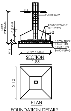
FOUNDATION DETAILS
