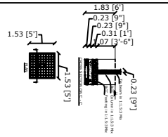
SECTION OF 20 FEET ROAD
