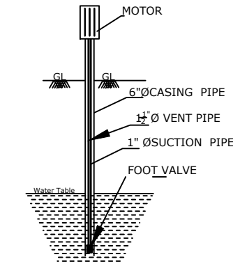
SEC. OF BOREWELL
