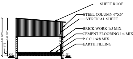
SECTION ON X-X
