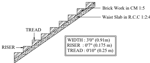
STAIRCASE DETAILS
