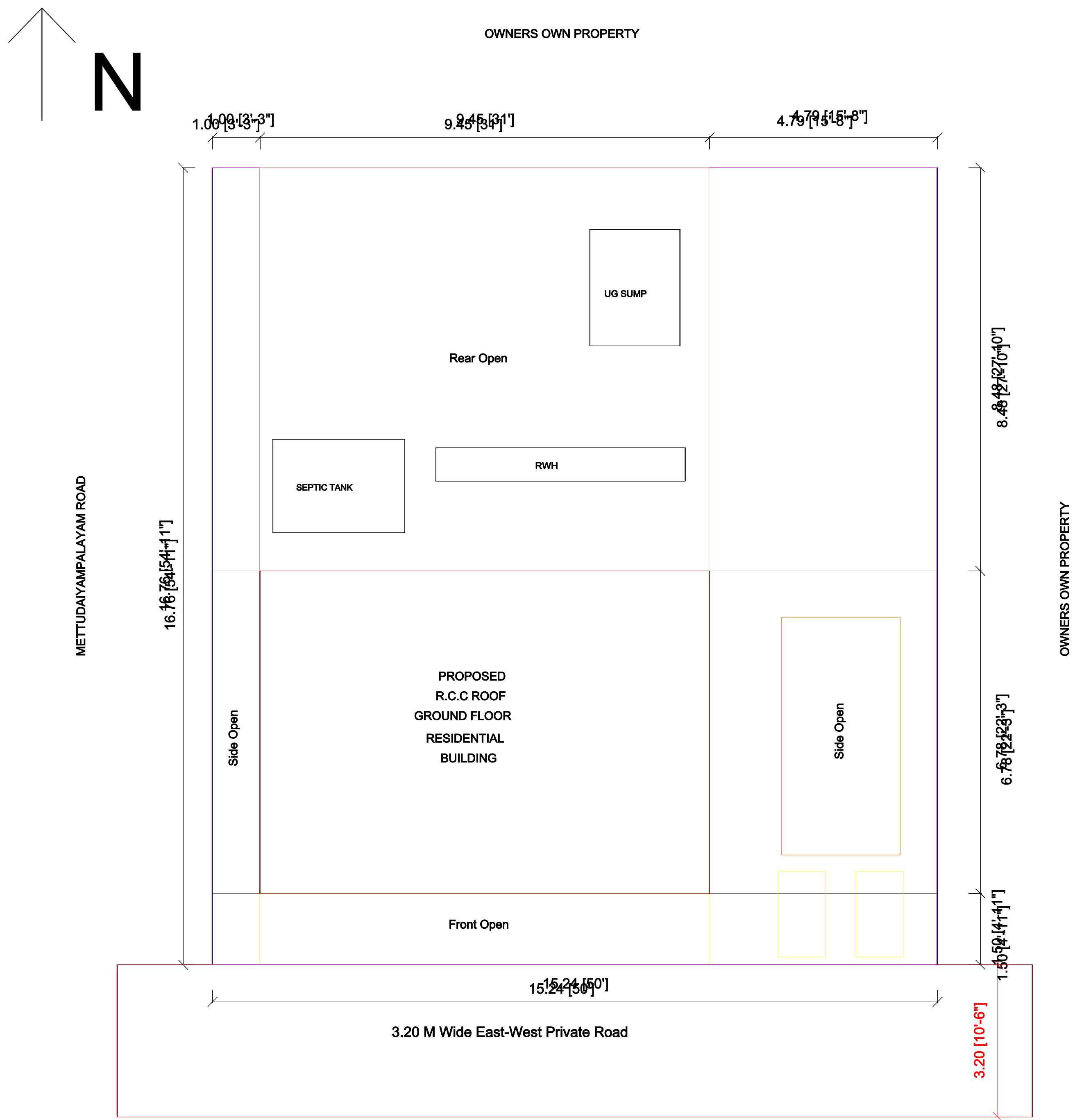
SITE PLAN
