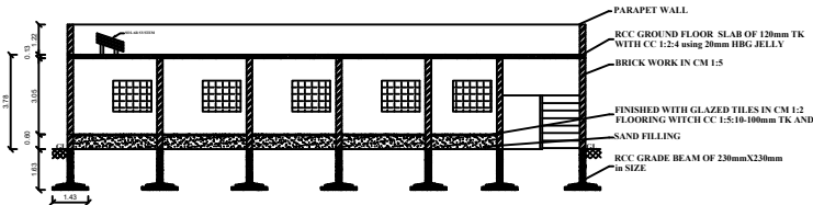
SECTION ON "AB"
