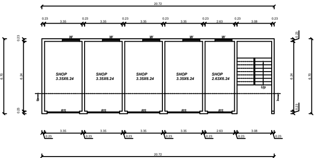
PROPOSED GROUND FLOOR PLAN [ NORTH FACING ]
