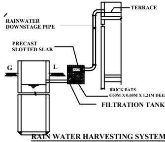
RAIN WATER HARVESTING SYSTEM
