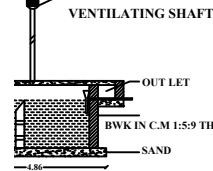
SEPTIC TANK
