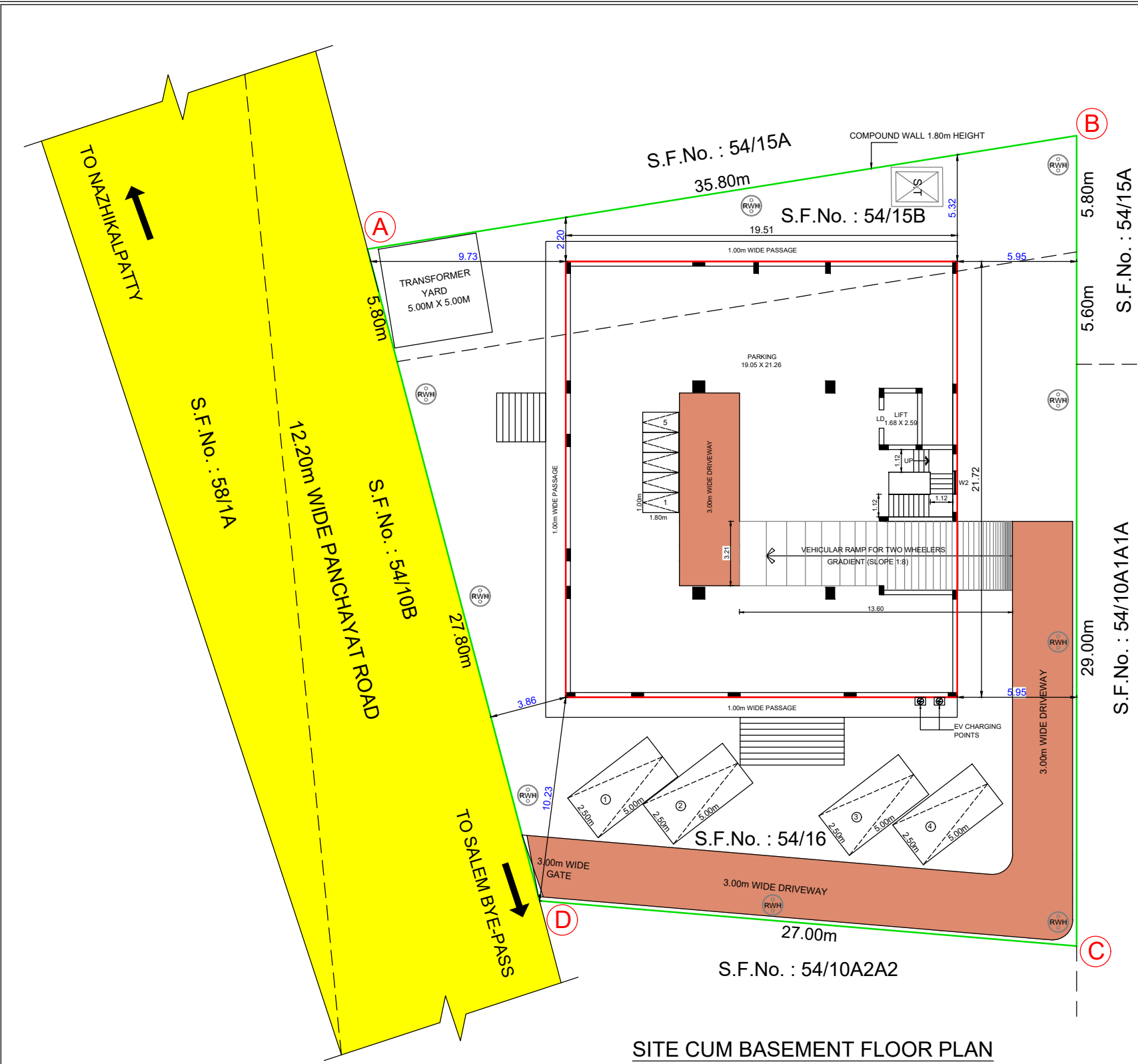
SITE CUM BASEMENT FLOOR PLAN
