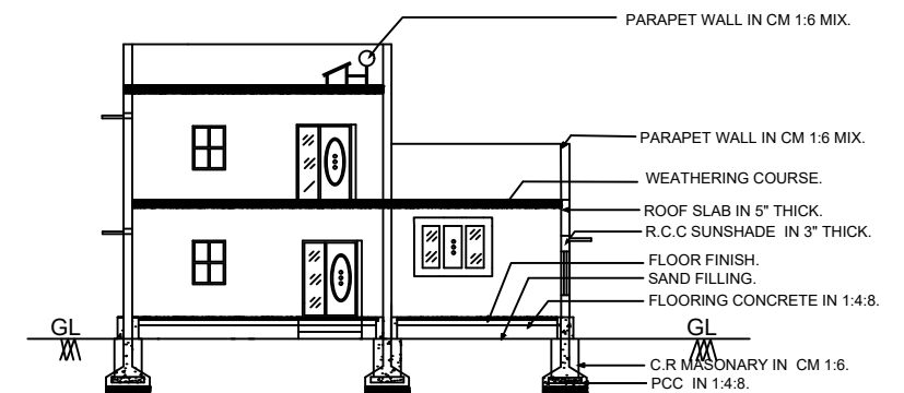
SECTION ON-AA
