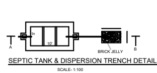
SEPTIC TANK & DISPERSION TRENCH DETAILS
