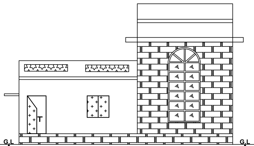
FRONT ELEVATION
