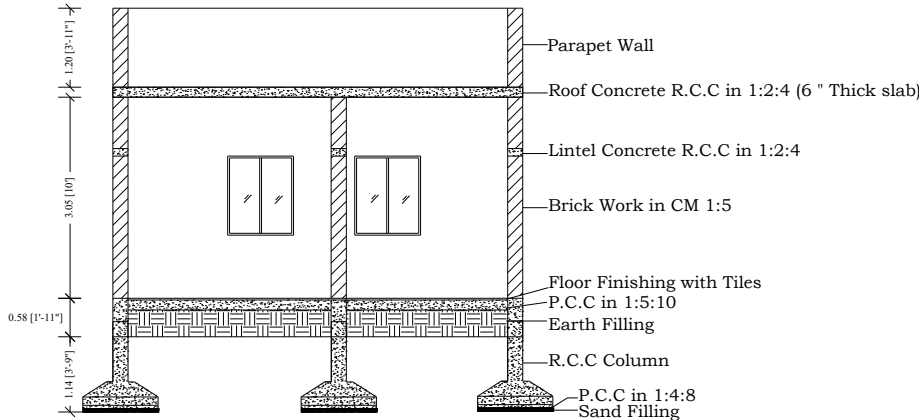
SECTION X-X
