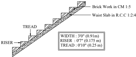
STAIRCASE DETAILS
