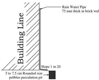
RAINWATER HARVESTING
