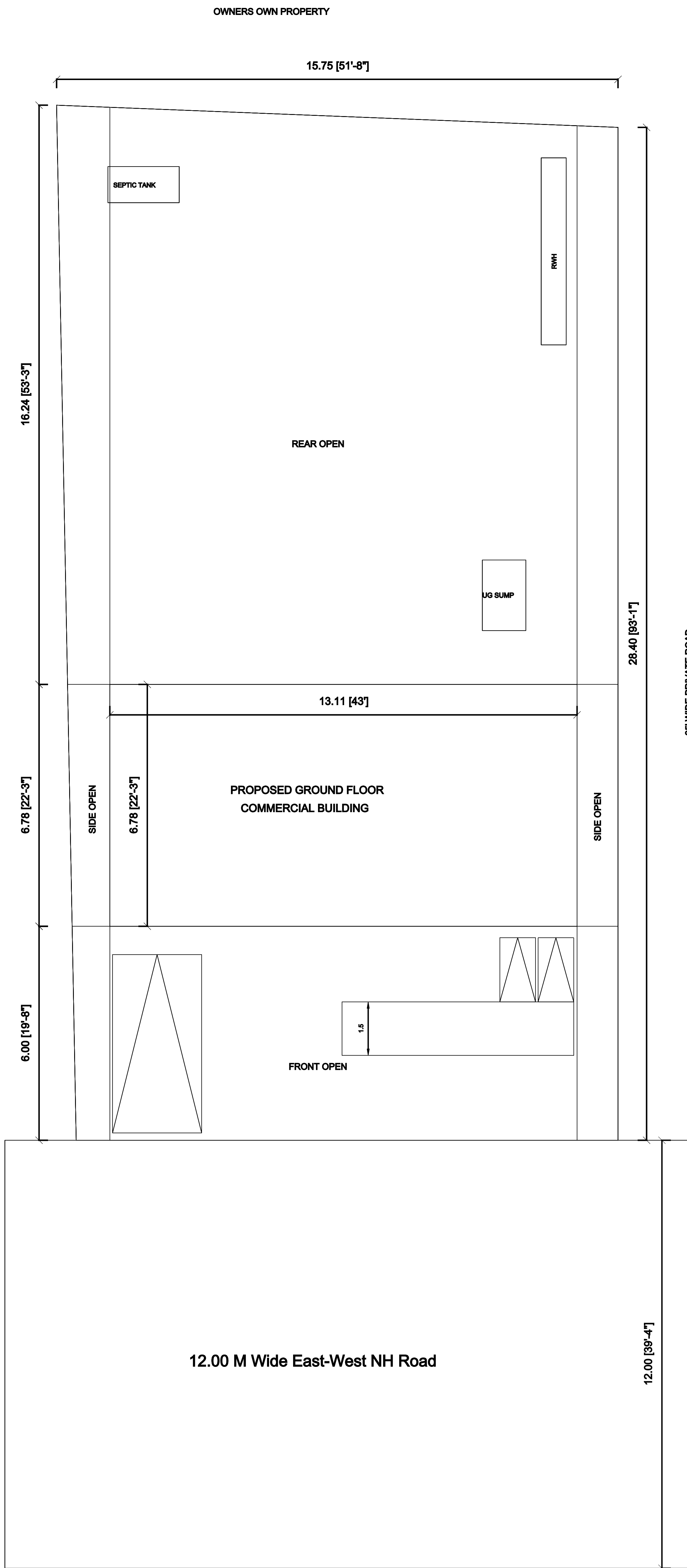
SITE PLAN
