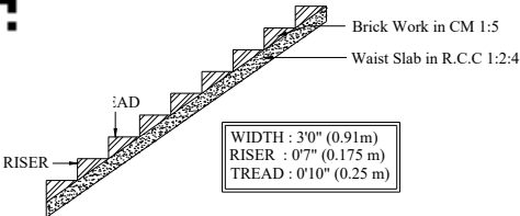
STAIRCASE DETAILS
